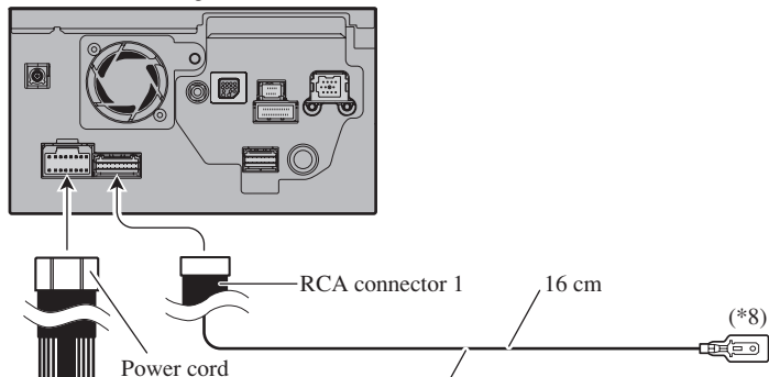
The navigation unit
